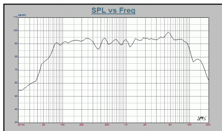
AЧХ (1Вт/ 1м) / RESPONSE CURVE (1w/1m)
