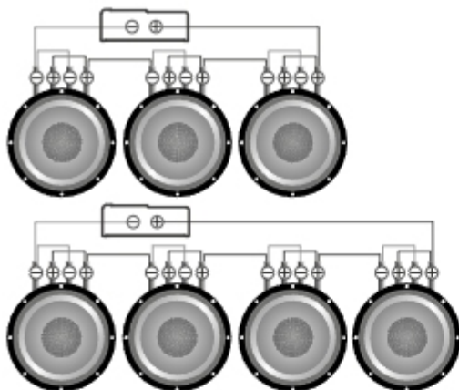
Subwoofers in series, coils in series
