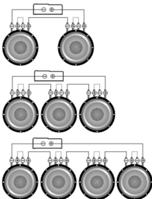
Subwoofers in parallel, coils in series
