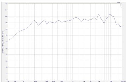
АЧХ (1Вт/ 1м) / RESPONSE CURVE (1w/1m)
